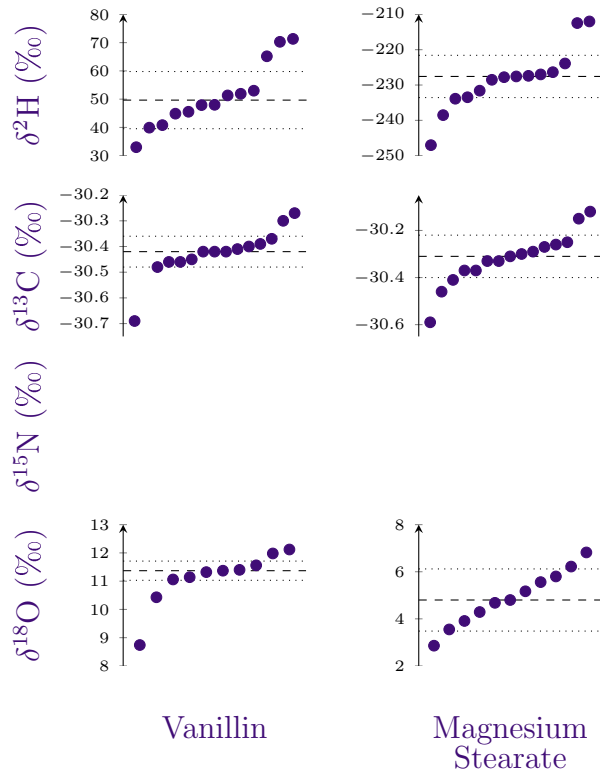
Results from FIRMS PT scheme Round 216. The lines represent the median of the results (dashed) plus or minus the robust standard deviation (dotted) following the exclusion of outliers.
